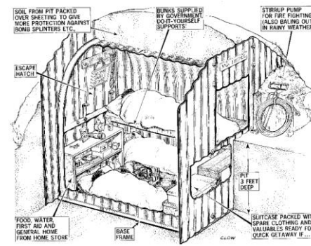
Cross-sectional diagram
